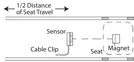
FIGURE 1a: SENSOR & MAGNET INSTALLATION (Sensor Installed on Centerline of Seat)
