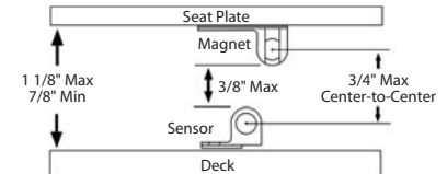
FIGURE 2: SENSOR & MAGNET SPACING
