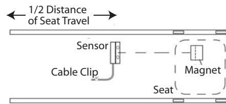
FIGURE 1b: SENSOR & MAGNET INSTALLATION (Sensor Offset Centerline of Seat)
